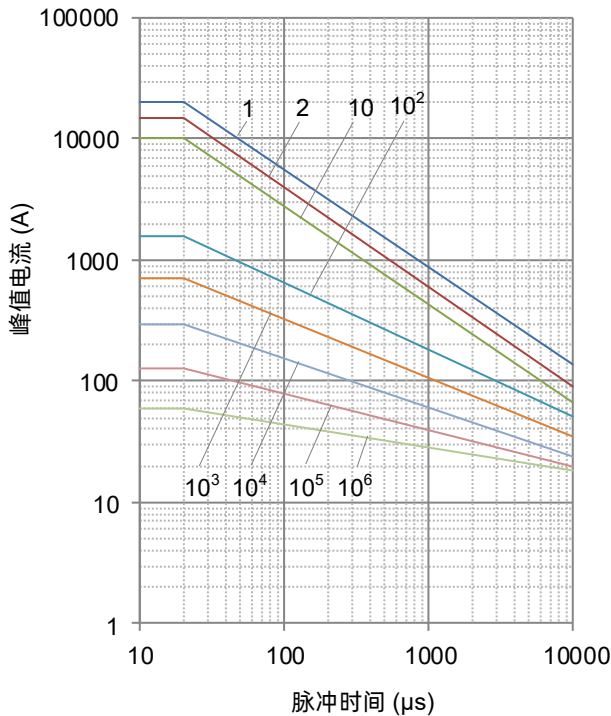
TFMOV34S470L to TFMOV34S680L
