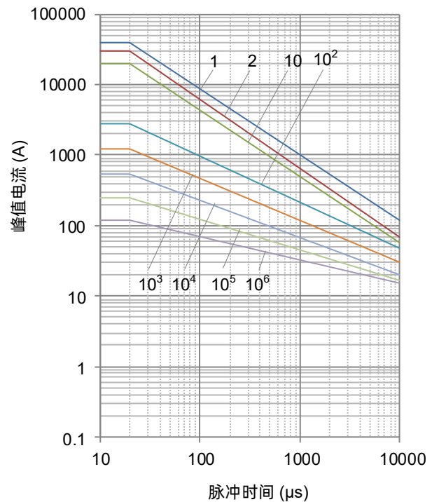
TFMOV34S820L to TFMOV34S681L
